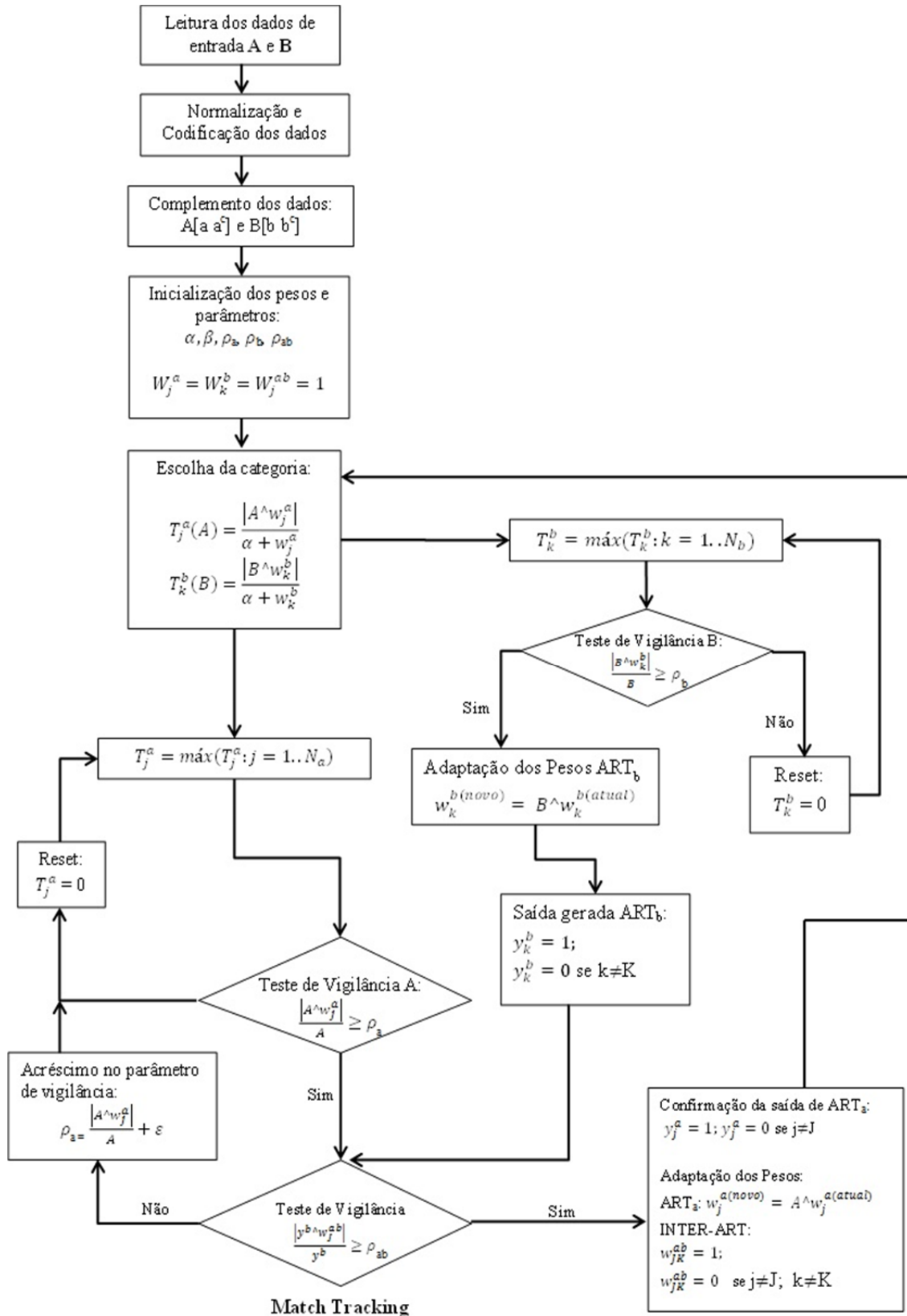
Fig. 2. Fluxograma da rede neural ARTMAP Fuzzy [11].
