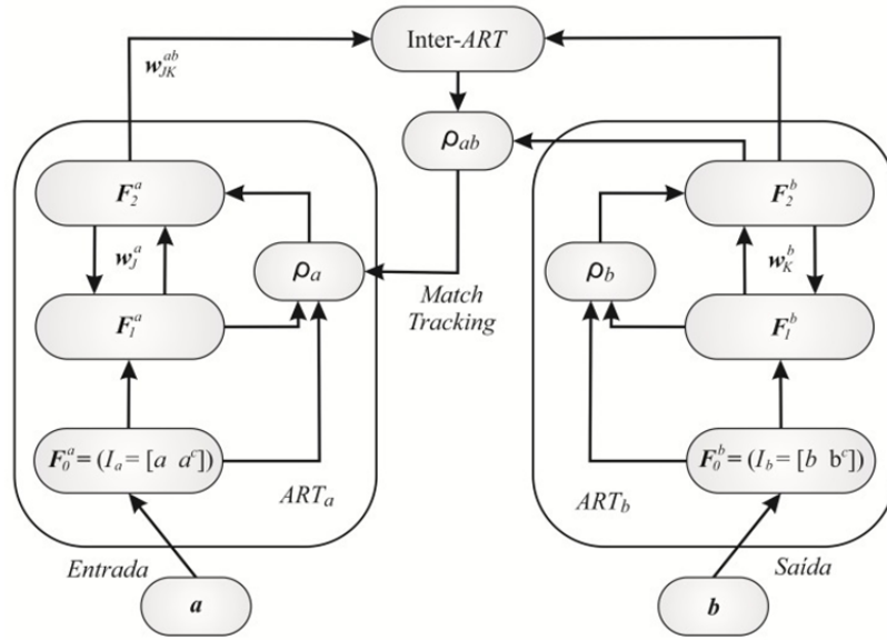
Fig. 1. Rede neural ARTMAP Fuzzy [2].
